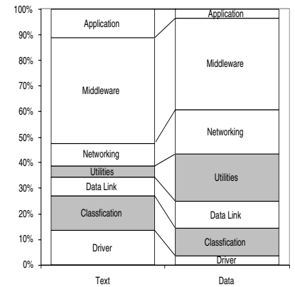
Fig. 5. Memory Layout
